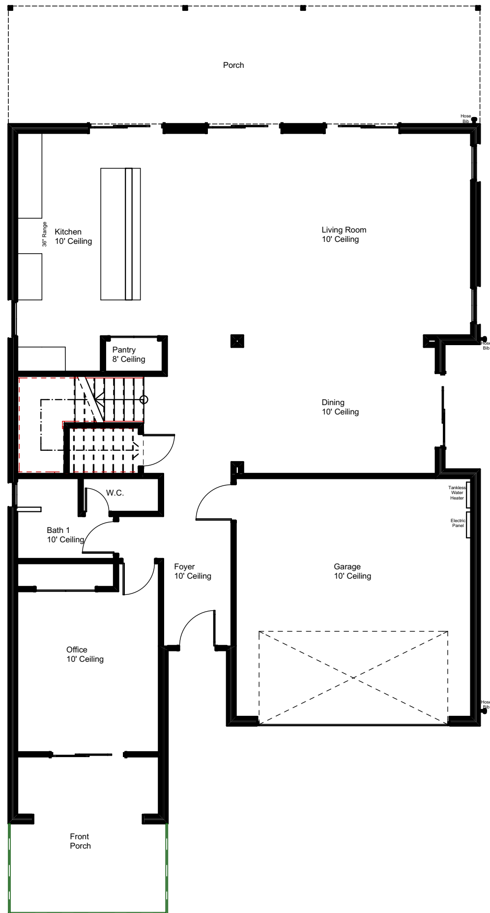
1 1st FLOOR SCALE: 1/8" = 1'-0"
