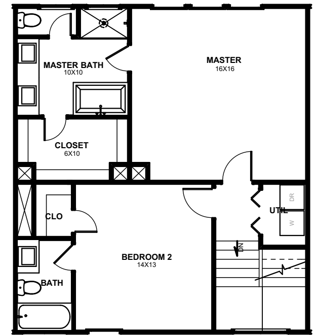
THIRD FLOOR
