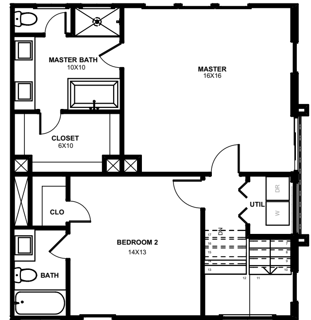
THIRD FLOOR
